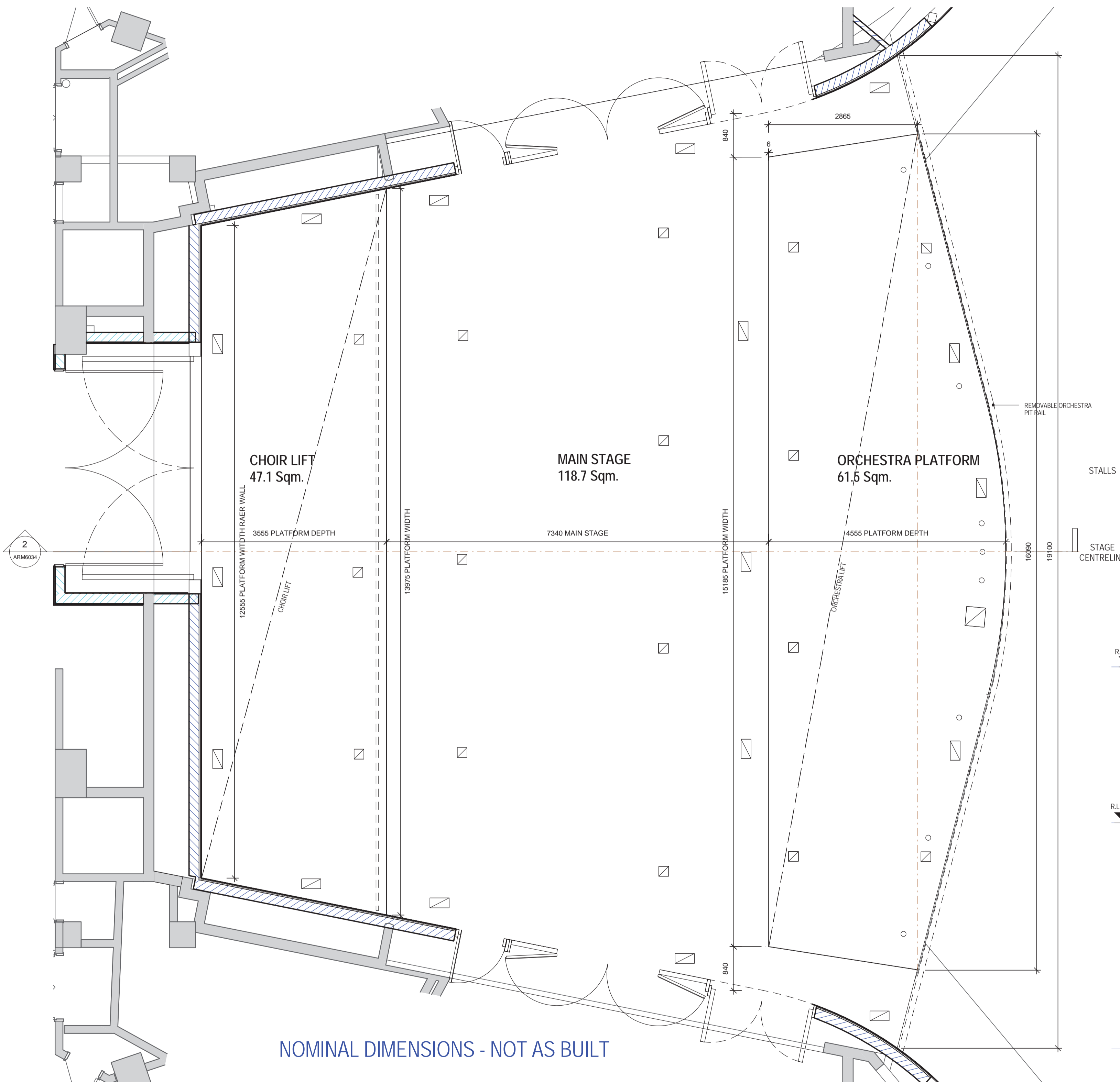
1 STAGE PART PLAN A110200 1:50
