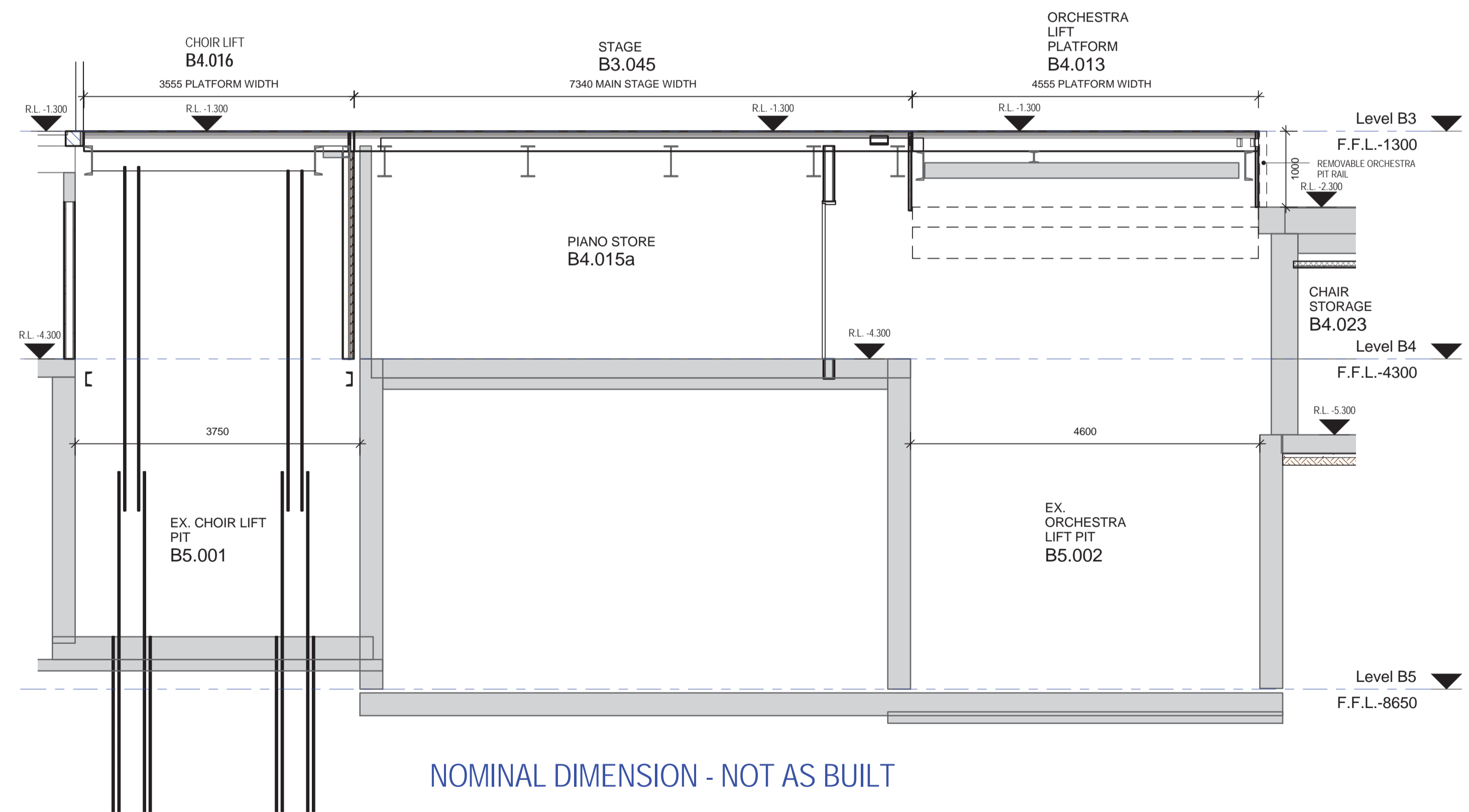
2 Section - Stage Setout A094002 1:50
